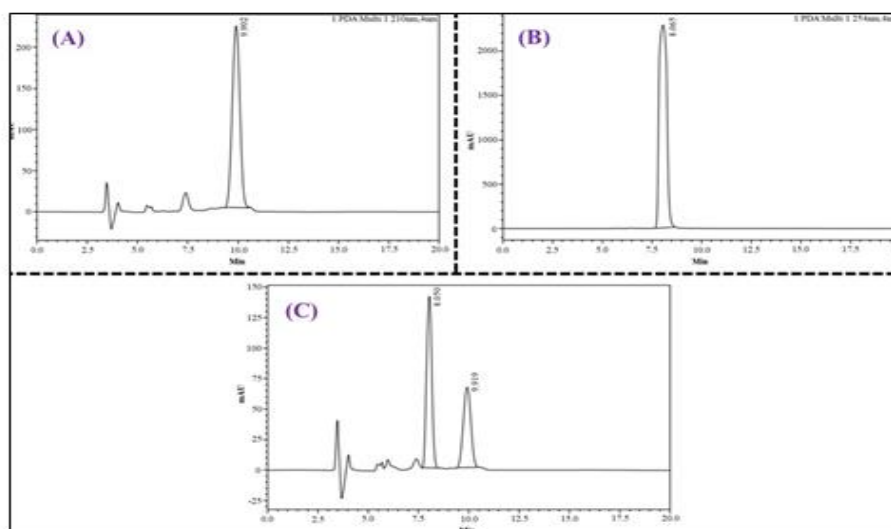
Figure 5: Representative RP-HPLC chromatogram of (A)TAC (B) THQ (C) THQ for simultaneous estimation.
