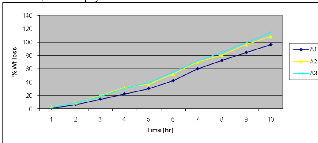
Figure 16. Erosion of batch A1, A2 an A3
