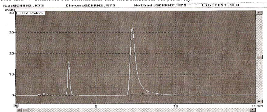
Figure 13. Chromatograph of amoxicillin and metronidazole
