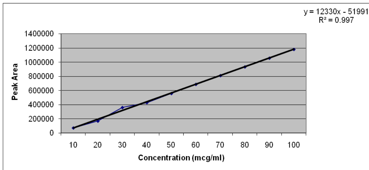
Figure 12. Calibration curve of metronidazole using HPLC method
