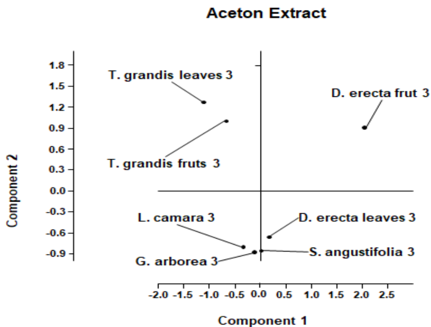
Fig. 8. Independent variables correlated with PCA factors F1 and F2.
