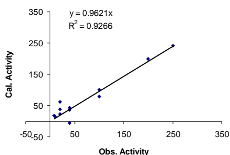
Fig. 2.1: Graph between observed and calculated MIC of thiophene group
