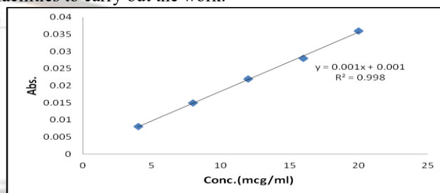
Fig. 1: Calibration curve of VAL
