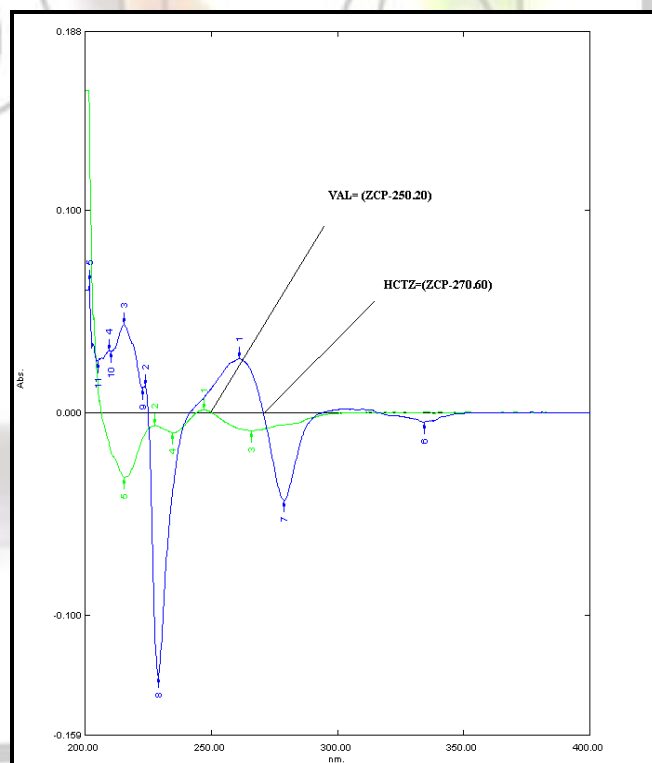
Fig. 3: Overlain First order Derivative absorption spectra of VAL and HCTZ in methanol
