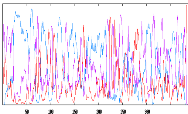
Fig. 2: Secondary structure prediction of Chlamydomonas reinhardtii by using GORIV method
