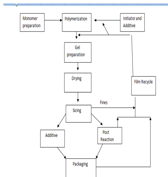
Block diagram of preparation of Hydrogel [17]
