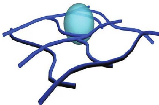
Fig. 1: Hydrogel Network [6]
