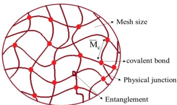
Fig. 1: Hydrogel Network [6]
