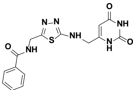
Fig. 1: Uracil substituted hippuric acid based 1,3,4-thiadiazole
