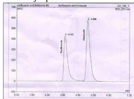
Figure 1: Chromatogram of standard solution of Norfloxacin-Tinidazole.
