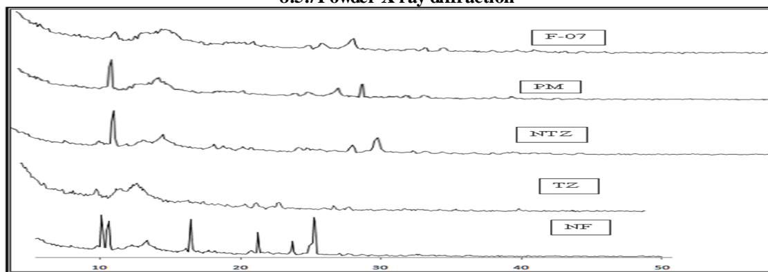
Figure 8.13: Overlain X-ray diffraction spectra of Norfloxacin, Tinidazole, Norfloxacin-Tinidazole combination, Physical mixture and optimized formulation.
