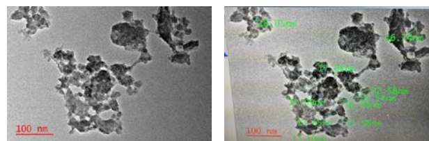
Fig 6: The Image of Cu nanoparticle synthesized using an aqueous extract of S. acidum
