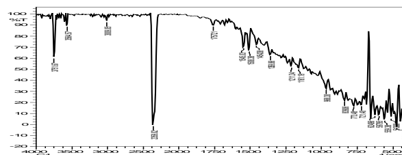
Fig 3: FTIR spectrum of copper nanoparticles synthesized using S. acidum
