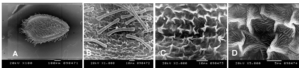
Fig. 2. Scanning electron micrographs: B. sylvestris var. cyrenaica A. Cypselae, B. bristles, C-D. Surface ornamentation
