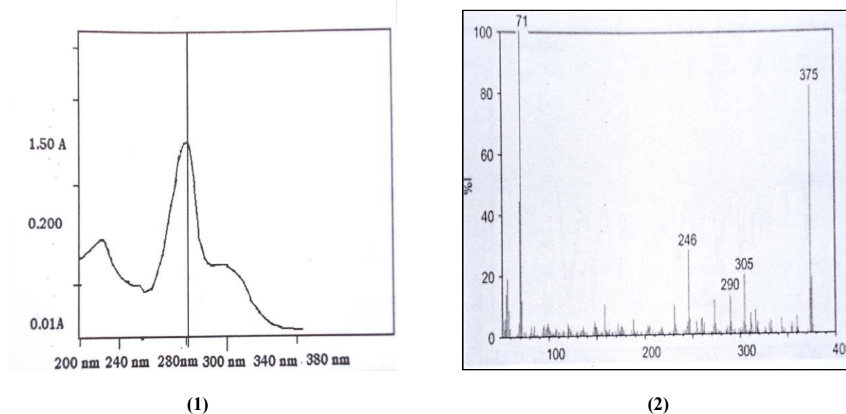
Fig. 1 : Absorption maxima ( \lambda_{\text{max}} )/wavelength maxima of ofloxacin
